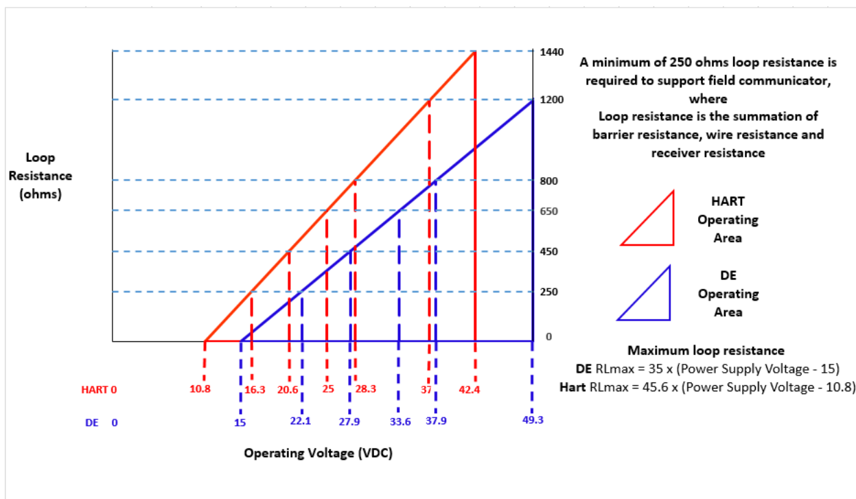
Figure 2 - Supply voltage and loop resistance chart &amp; calculations
