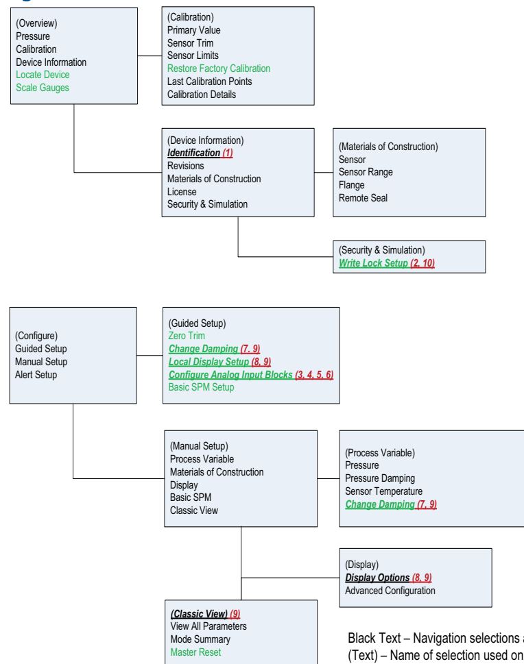
Figure 2-11. Partial Menu Tree
