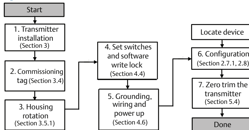
Figure 1-1. FOUNDATION fieldbus Installation Flowchart
