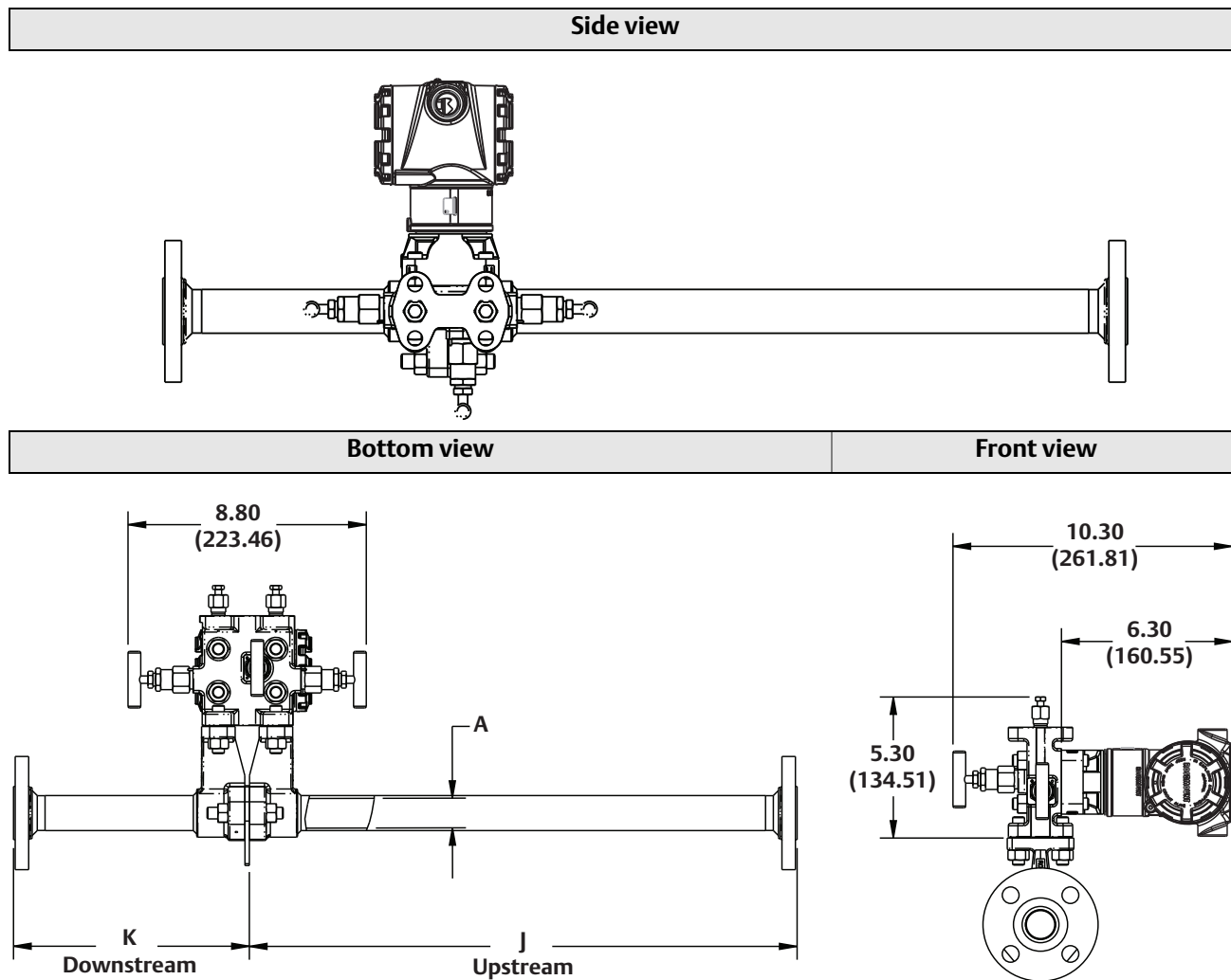
Figure A-16. Rosemount 3051CFP Integral Orifice Flowmeter
