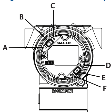
Figure 4-2. Simulate and Security Switches
