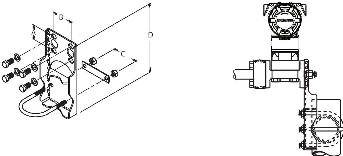
Figure 3-8. Flat Mounting Bracket Option Codes B3 and BC
