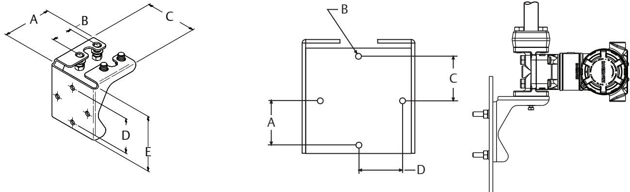
Figure 3-7. Panel Mounting Bracket Option Codes B2 and B8
