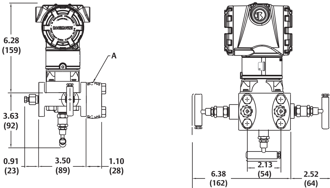
Figure A-8. Rosemount 3051C Coplanar with Rosemount 305RT3 3-Valve Traditional Integral Manifold
