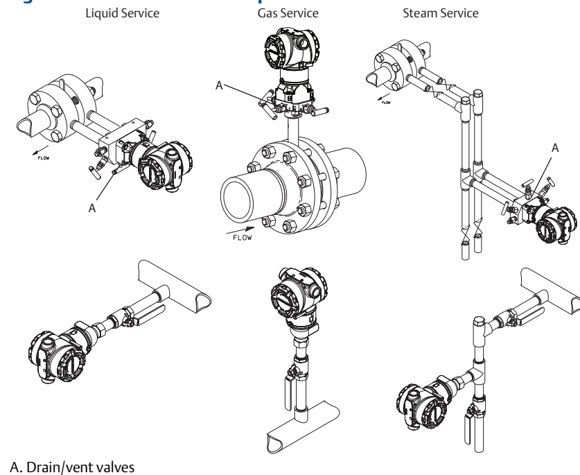
Figure 3-10. Installation Examples
