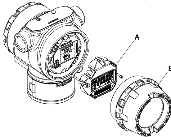
Figure 4-1. LCD Display Assembly
