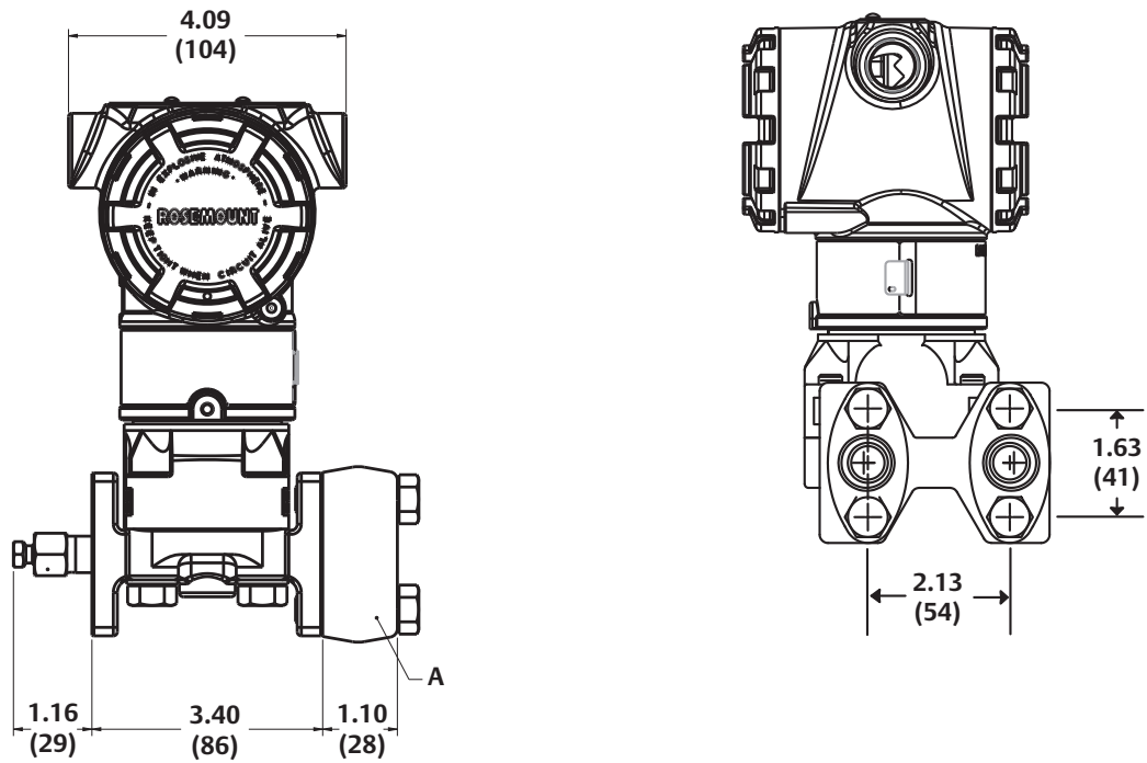
Figure A-7. Rosemount 3051C Coplanar with Traditional Flange
