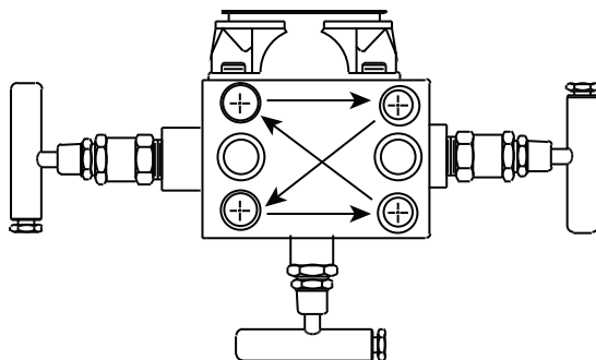
Figure 3-14. Bolt Tightening Pattern
