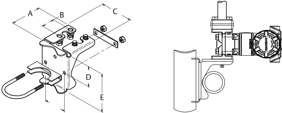
Figure 3-6. Mounting Bracket Option Codes B1, B7, and BA
