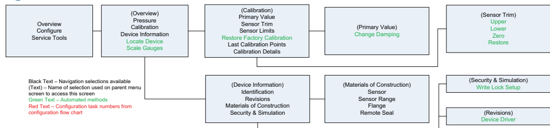
Figure 2-4. Overview Section of the Menu Tree
