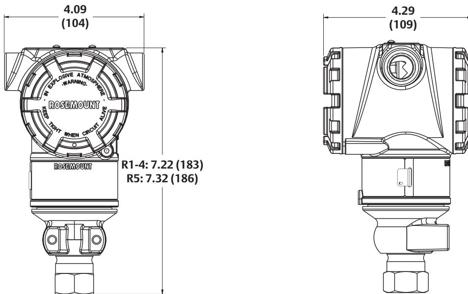
Figure A-10. Rosemount 3051T Dimensional Drawings
