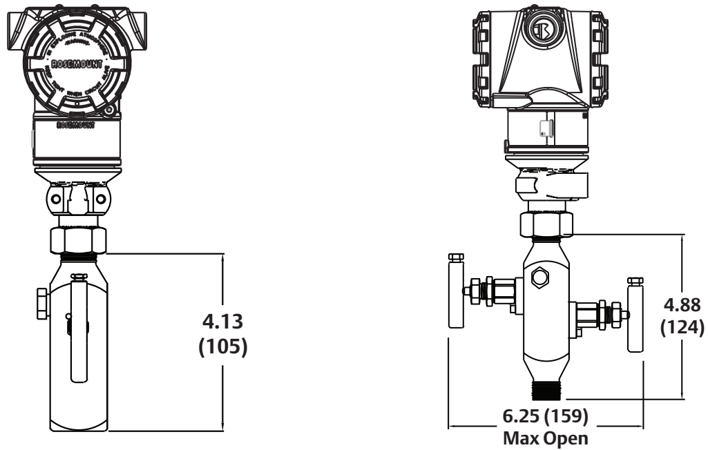
Figure A-12. Rosemount 3051T with Rosemount 306 2-Valve I Integral Manifold
