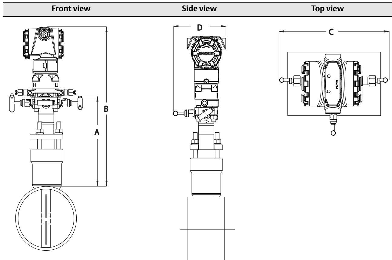
Figure A-14. Rosemount 3051CFA Pak-Lok Annubar Flowmeter (1)
