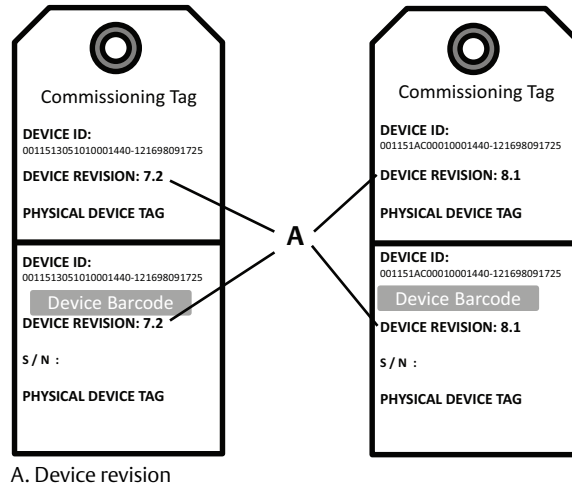
Figure 3-1. Commissioning Tag
