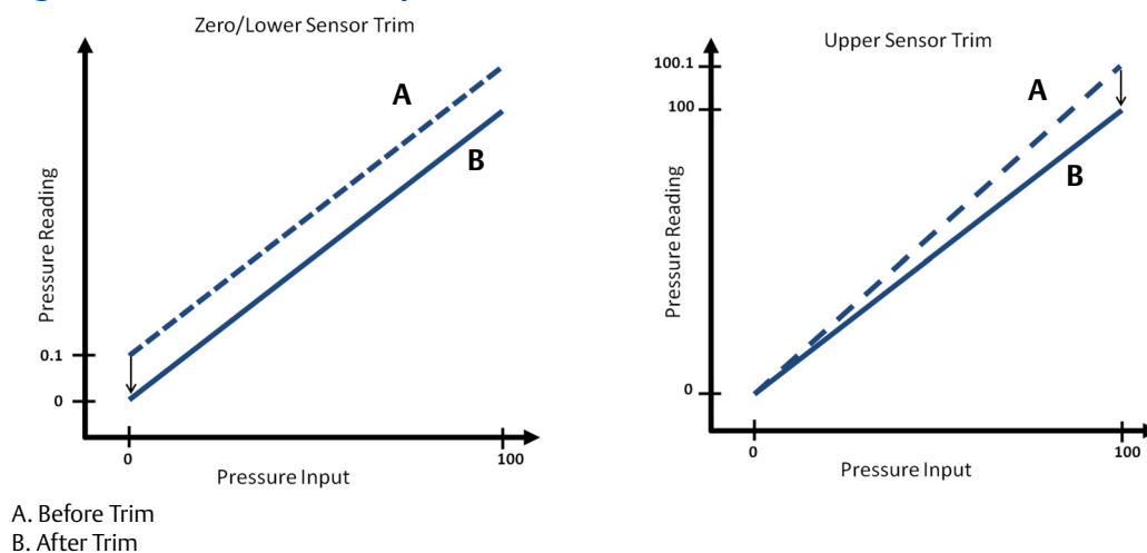
Figure 5-1. Sensor Trim Example
