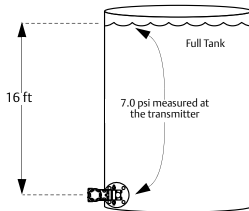
Figure 2-16. Situation #2 Diagram
