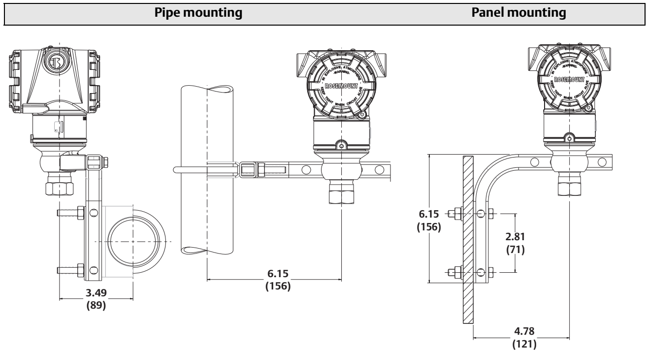
Figure A-13. Rosemount 3051T Typical Mounting Configurations with Optional Mounting Bracket
