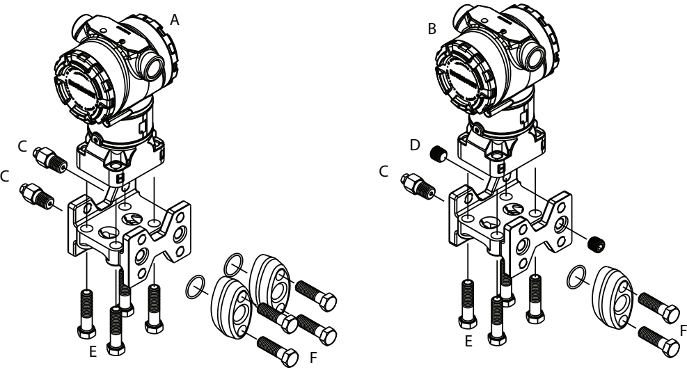
Figure 3-3. Traditional Flange Bolt Configurations
