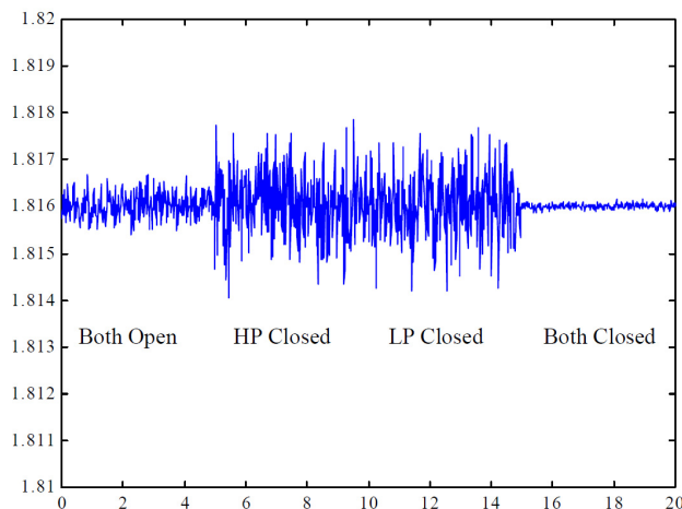
Figure 7-9. Differential Pressure Signals under Different Plugging Conditions
