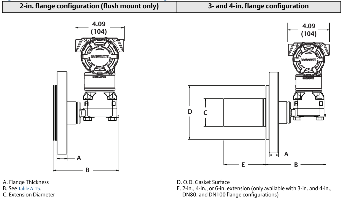
Figure A-17. Rosemount 3051L Dimensional Drawings
