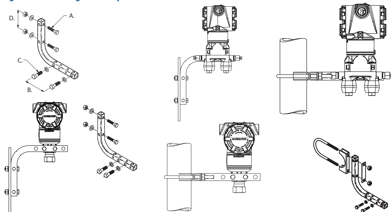
Figure 3-9. Mounting Bracket Option Code B4
