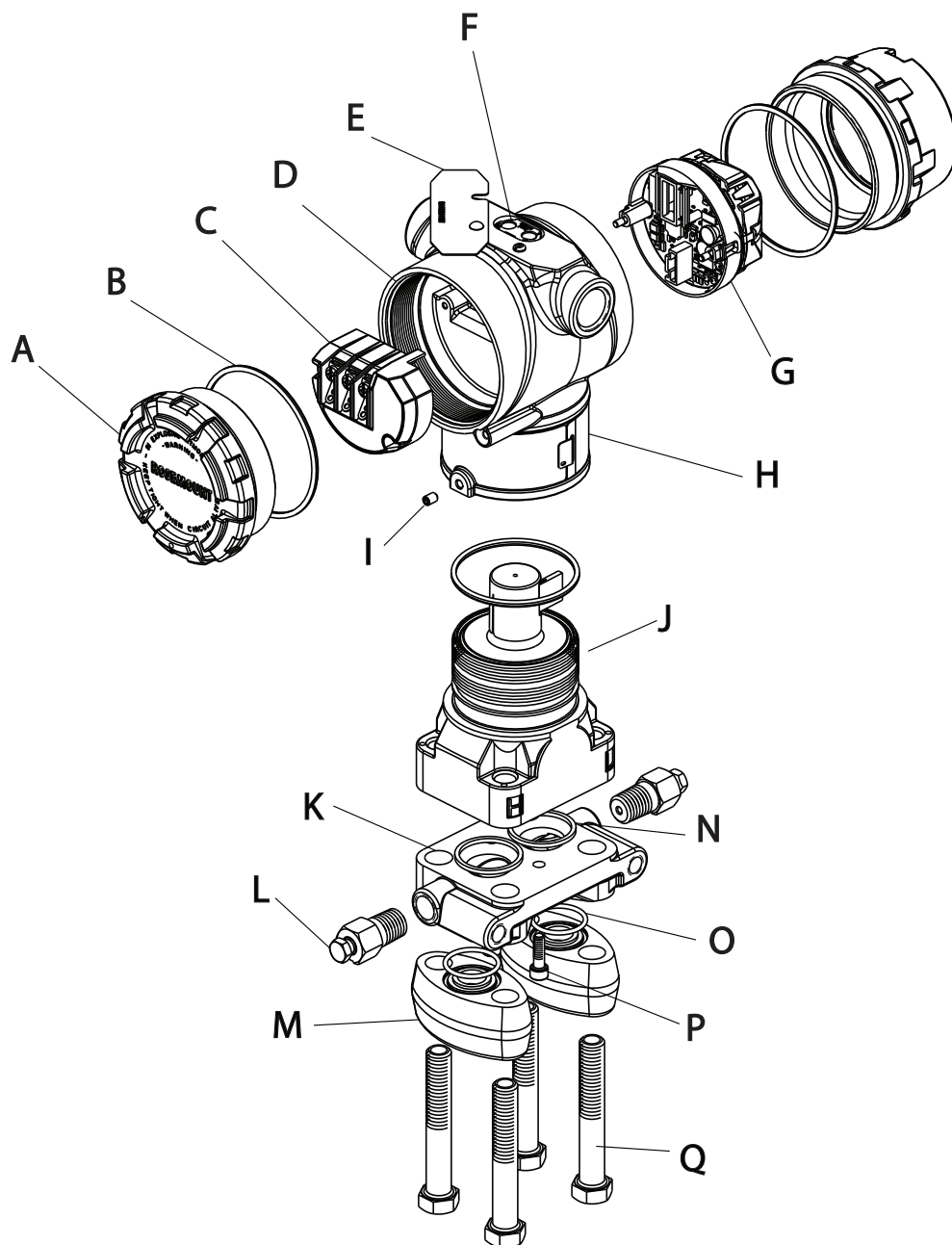
Figure A-2. Rosemount 3051C Exploded View
