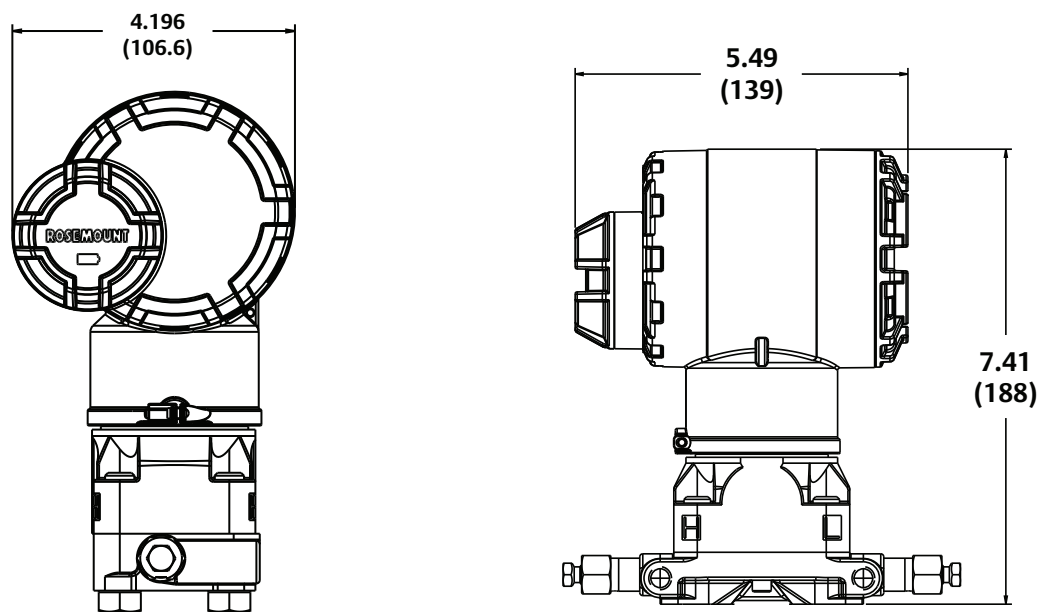
Figure A-4. 3051 Wireless Housing with Coplanar Flange
