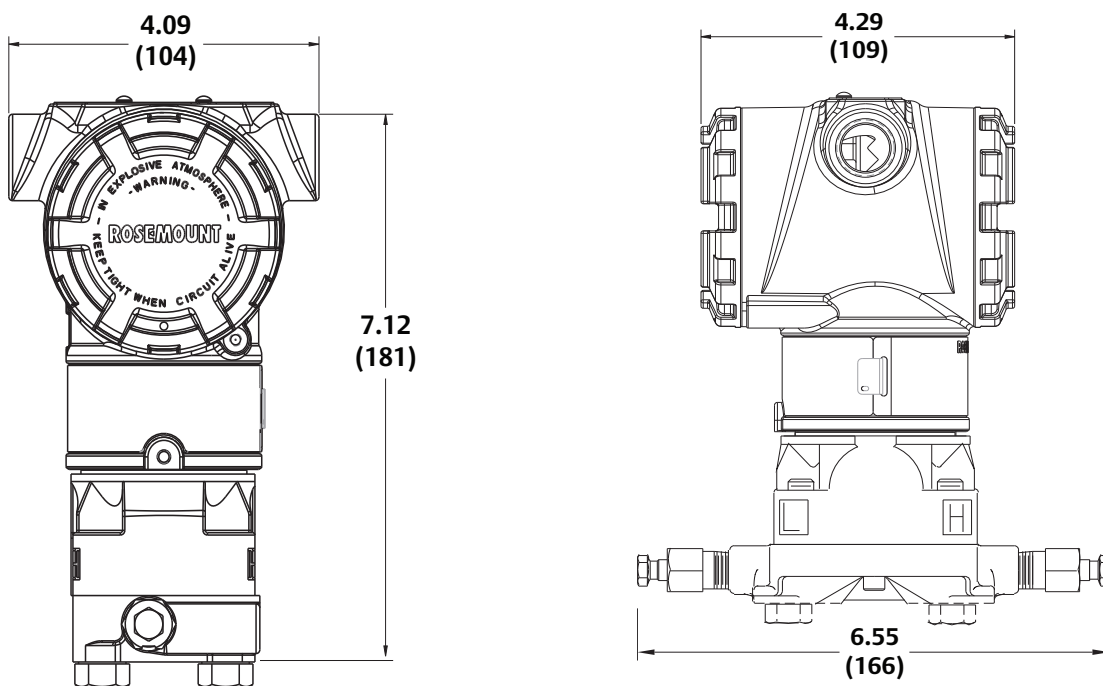
Figure A-3. Rosemount 3051C Coplanar Flange
