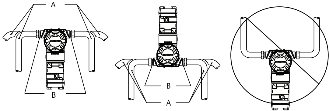
Figure 4-3. Conduit Installation Diagrams
