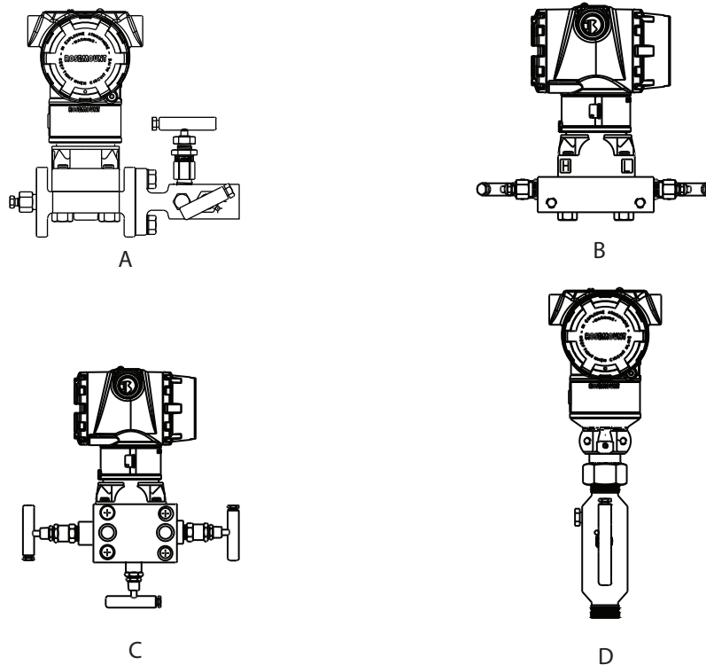
Figure 3-13. Manifolds
