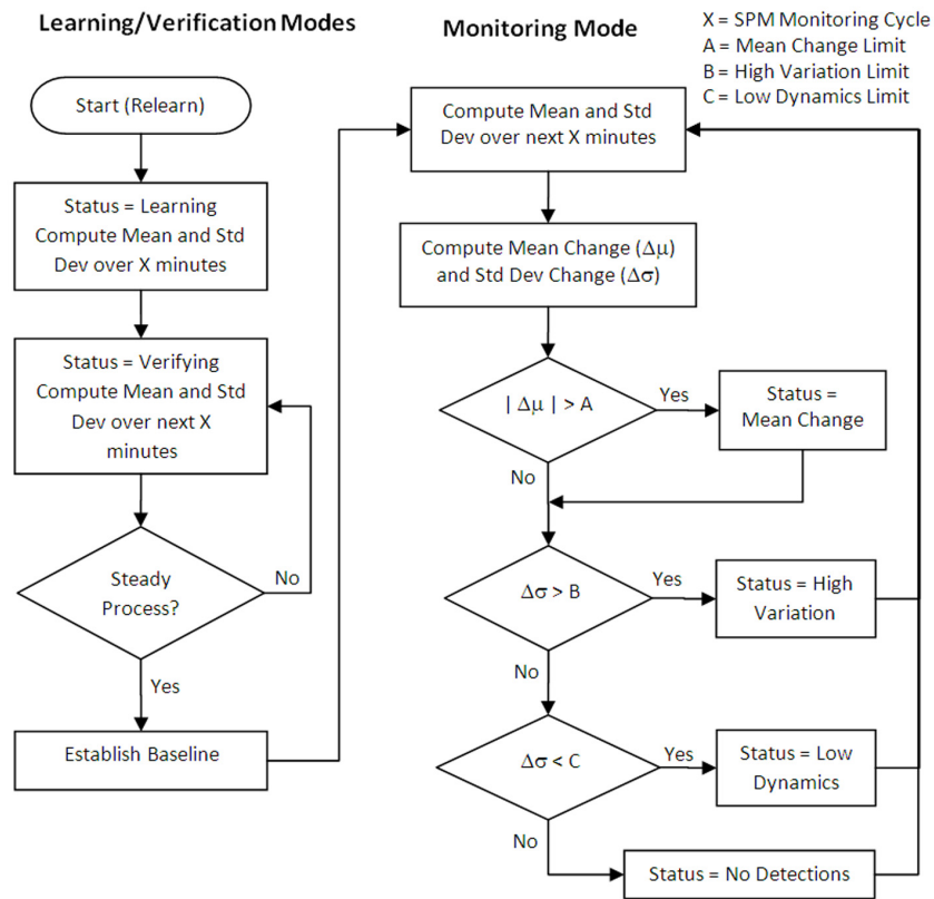
Figure 7-4. Flow Chart of 3051 FF SPM
