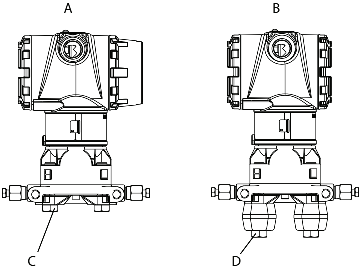
Figure 3-5. Mounting Bolts and Bolt Configurations for Coplanar Flange
