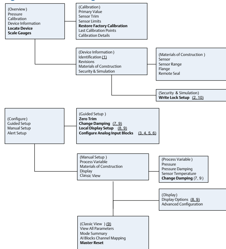
Figure 2-14. Basic Configuration Menu Tree
