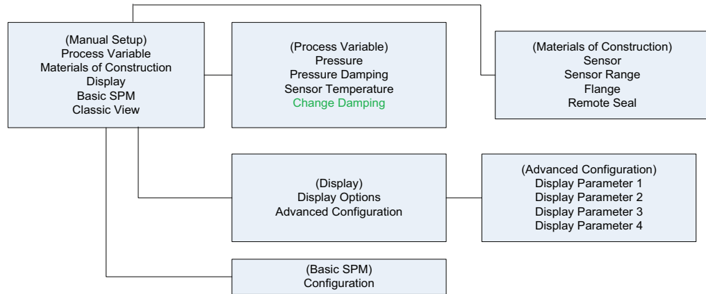
Figure 2-6. Manual Setup Branch of the Menu Tree
