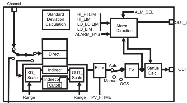
Figure A-1. AI Block Internal Components
