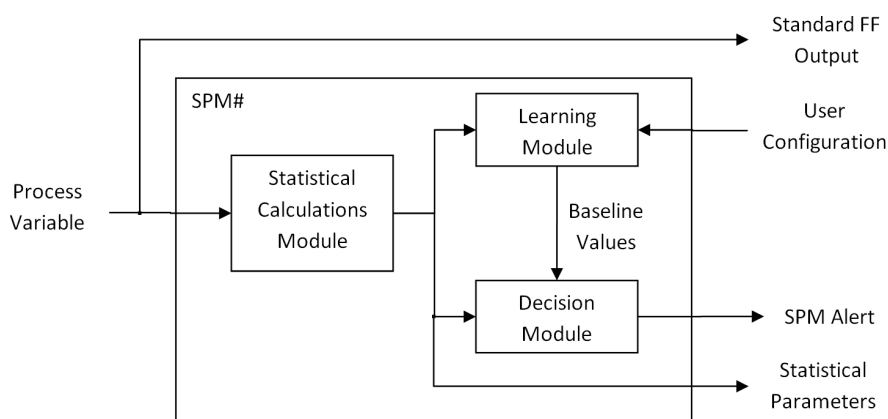
Figure 7-3. Diagram of 3051 FF Statistical Process Monitoring
