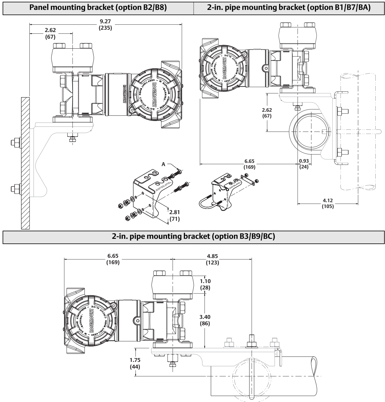
Figure A-9. Traditional Flange Mounting Configurations with Optional Brackets for 2-in. Pipe or Panel Mounting
