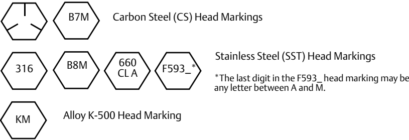
Figure 3-4. Head Markings
