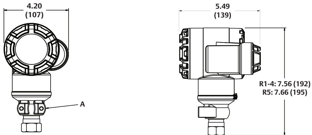
Figure A-11. 3051T Wireless Housing Dimensional Drawings
