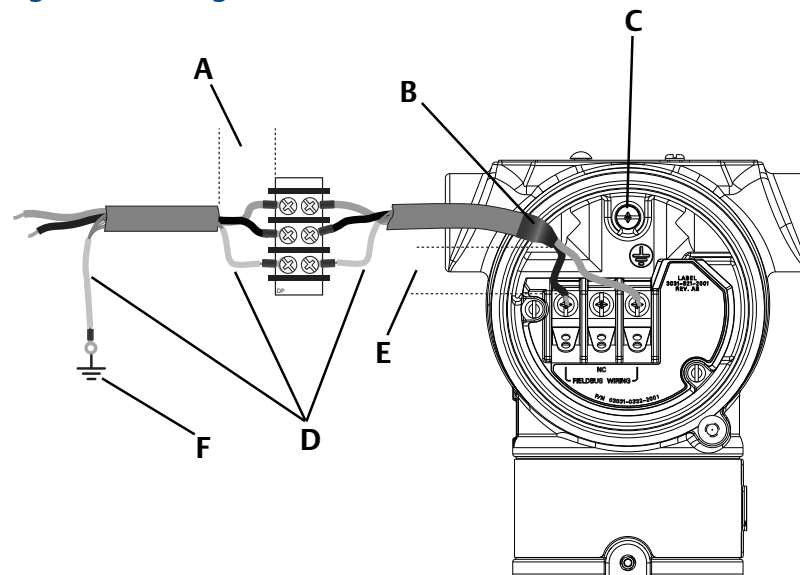
Figure 4-4. Wiring Terminals
