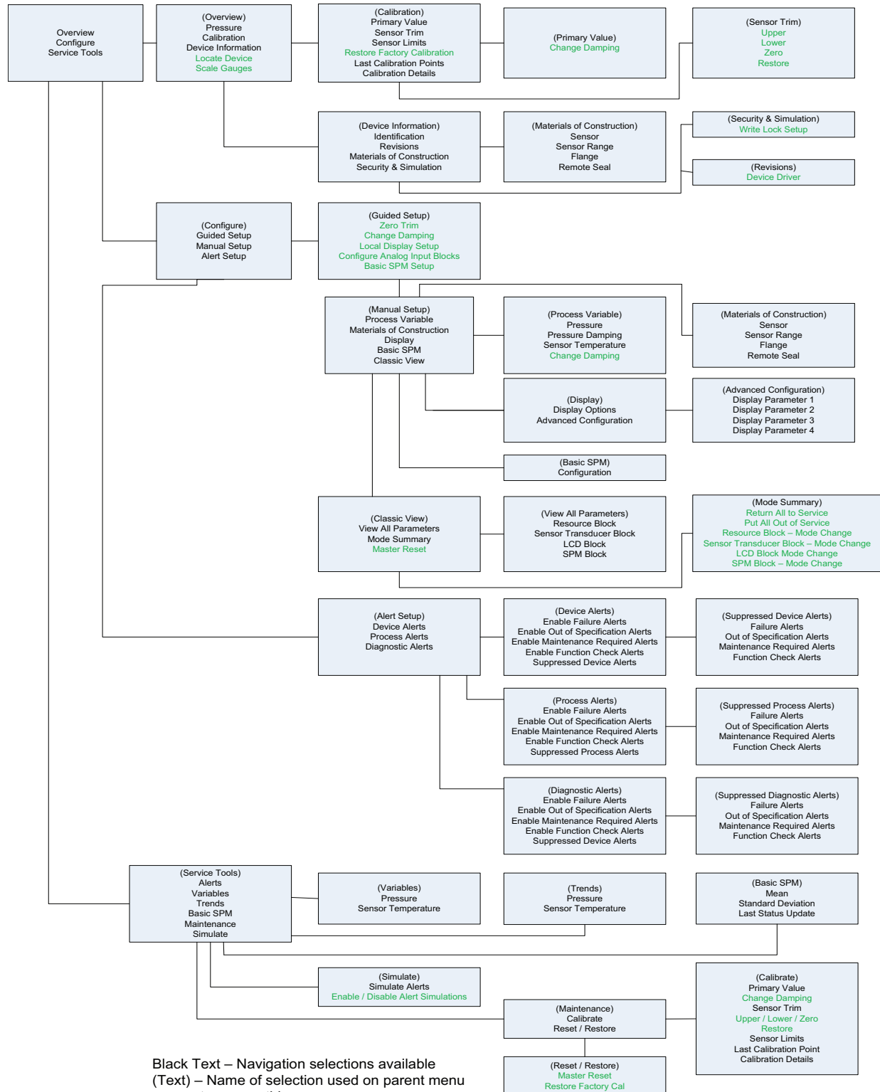
Figure 2-10. Complete Menu Tree
