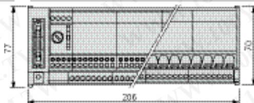
Sub-bases
