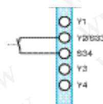
Manual reset without start button monitoring
