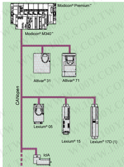
MFB: Motion control distributed over CANopen
