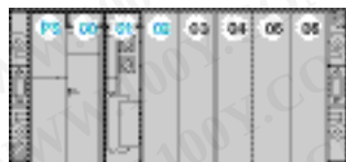
Principal rack address 0 with double format power supply and standard format processor
