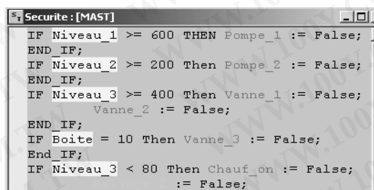
Animation of ST program
