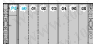
Extension rack address n with standard format power supply
