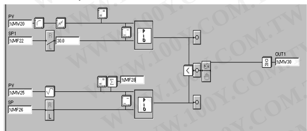
Autoselective loop
