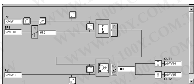
Cascaded loop
