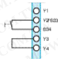
Manual reset with start button monitoring
